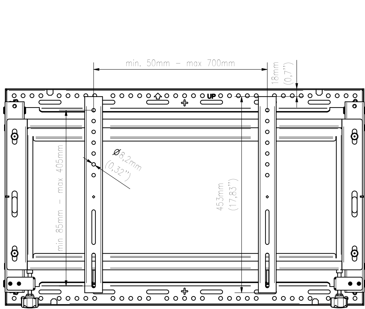
FRONT VIEW
